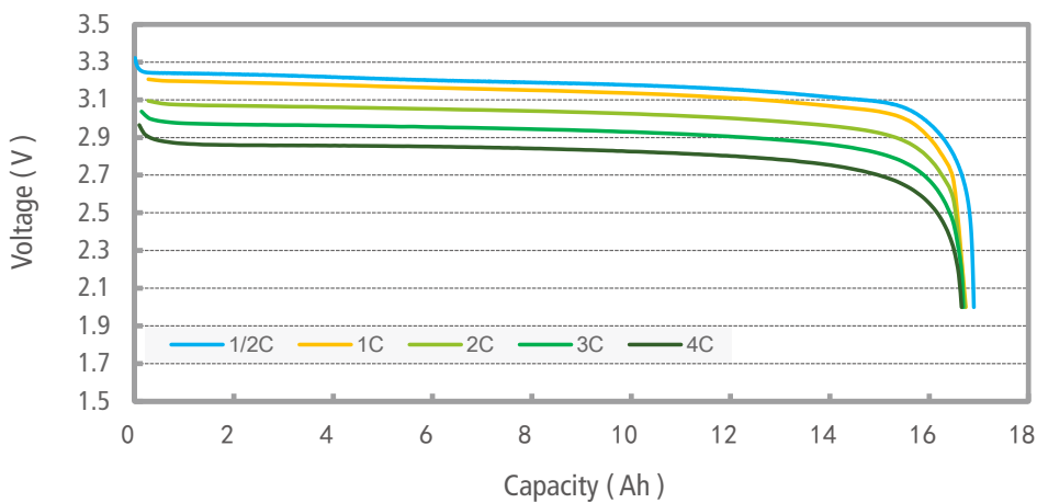
Discharge characteristic at 25°C
