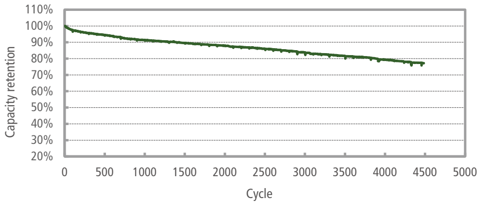
Cycle Life @RT 1C Charge And Discharge
