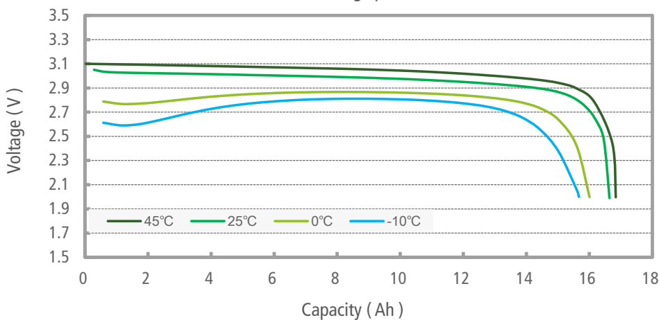
2C discharge performance
